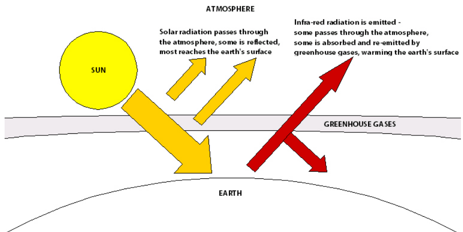
Figure 1.1: Greenhouse gas effect
