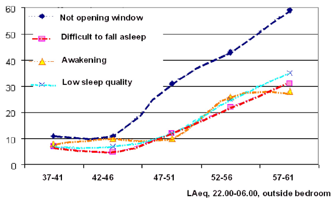
Figure 9. Results from Swedish Soundscape research program 20 .
