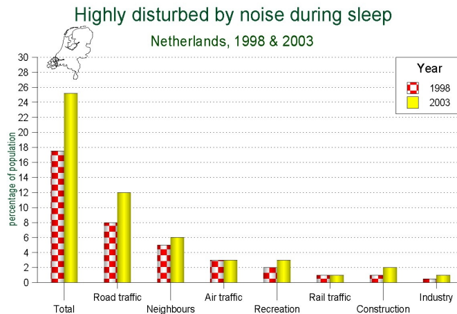
Figure 1. Percent of population stating to be highly disturbed by noise during night time (RIVM survey 2003 9 ).
