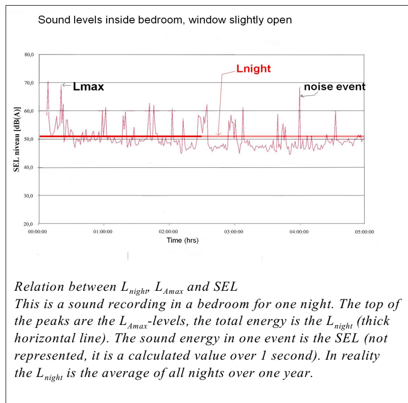
Figure 2 showing the relation between L_{\text{Amax}} , SEL and LAeq
