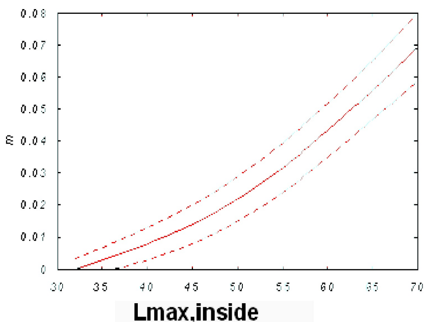
Figure 4. Probability of (aircraft) noise-induced motility ( m ) at the 15-s interval in which the indoor maximum sound level occurs (solid line) and the 95% confidence interval, as a function of L_{Amax,inside} bedroom (Passchier-Vermeer et al 18 , 2002).
