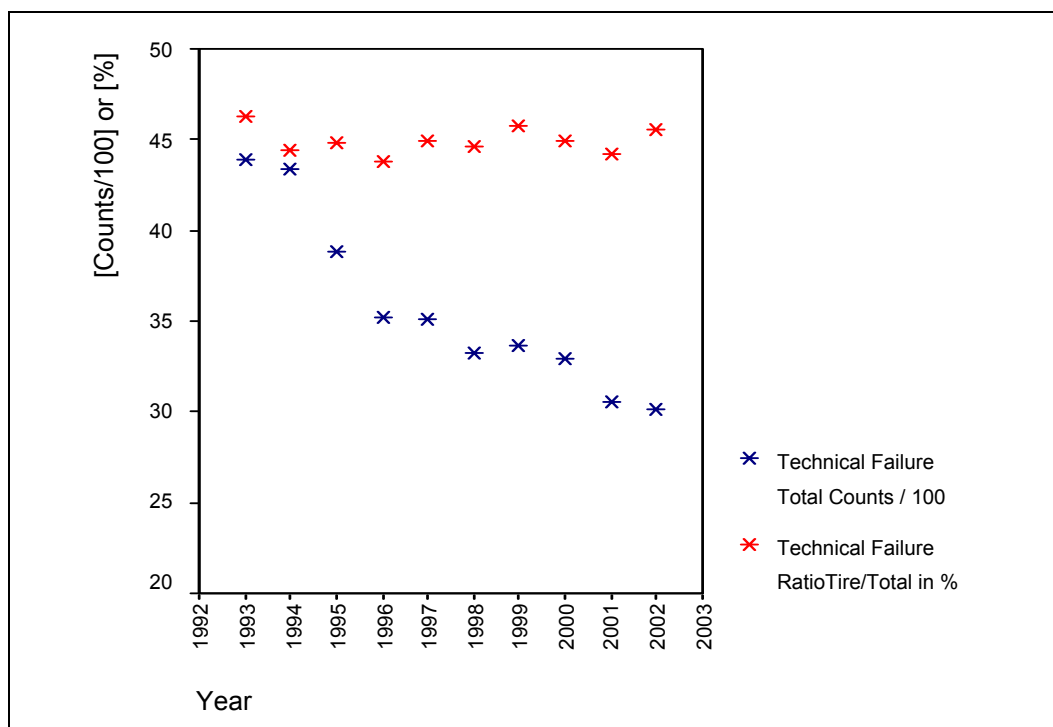
Fig. 2.1: Chronological development of tyre defects related to total technical failures in Germany
