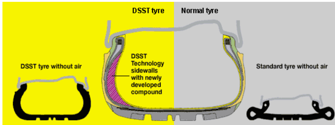
Fig. 3.1: Comparison of the sidewall construction between a normal and a run-flat-tyre (Example: Dunlop Self Supporting Technology DSST) [15]
