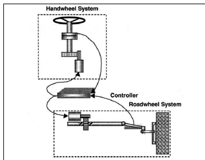
Fig. 3.13: Design of a steer-by-wire system [34]
