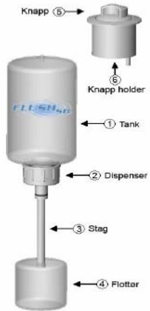
Figur 1: Flush systemet
