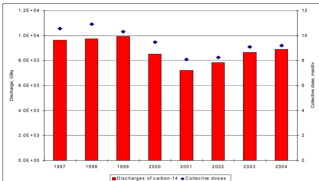
Figure 12 Reported liquid discharges of ^{14}\text{C} from Cap de la Hague and implied total collective dose to the EU population truncated at 500 y from exposure to all reported liquid discharges
