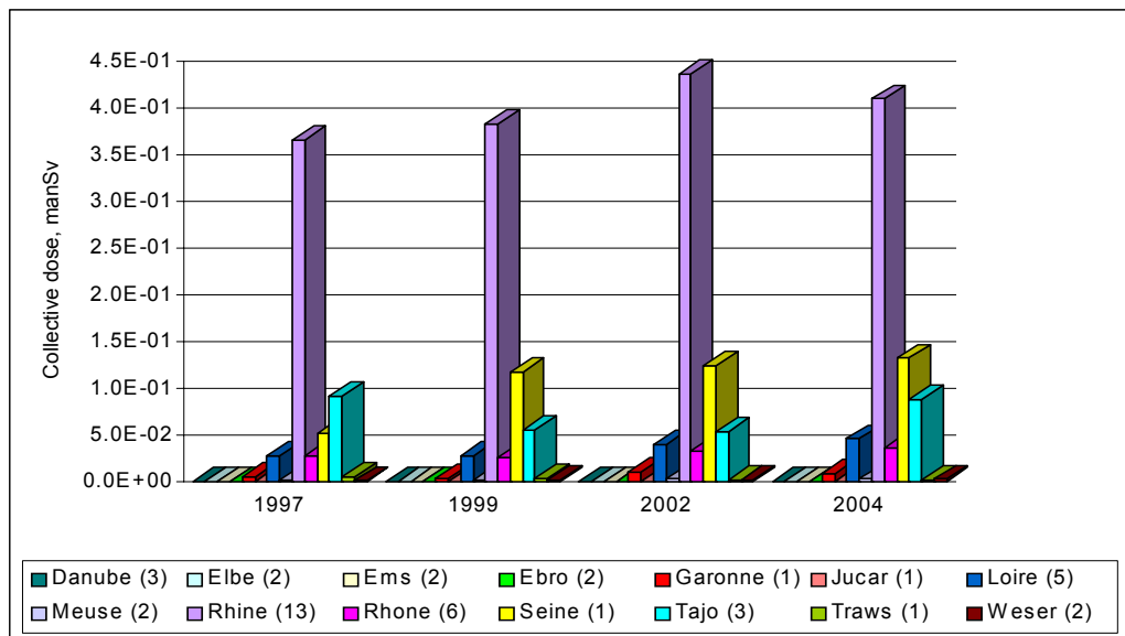
Figure 6 Implied collective doses truncated at 500 y to the EU population from drinking water as a result of reported discharges to rivers from inland sites. Legend includes number of sites in brackets
