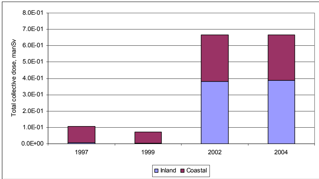
Figure 9 Implied collective doses truncated at 500 y to the EU population arising from reported marine discharges from all nuclear power stations (for some sites reported discharges did not include 14 C prior to 2002)
