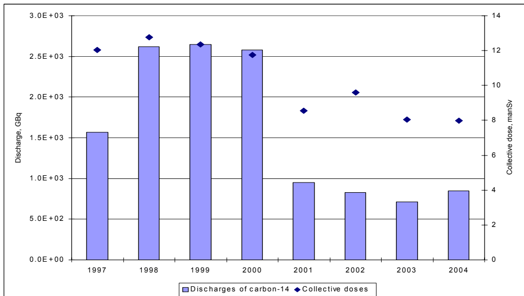
Figure 4 Reported atmospheric discharges of ^{14}\text{C} from Sellafield and implied total collective dose to the EU population truncated at 500 y from exposure to all reported atmospheric discharges
