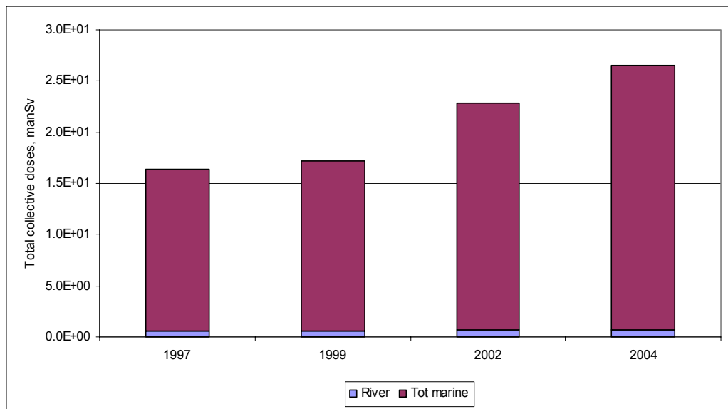
Figure 14 Implied collective doses truncated at 500 y to the EU population arising from reported river and marine discharges for all nuclear sites (for some sites reported discharges did not include ^{14}\text{C} prior to 2002)
