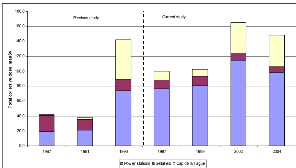
Figure 2 Implied collective doses to the EU population truncated at 500 y arising from reported atmospheric discharges from all nuclear power stations, Sellafield and Cap de la Hague (for Cap de la Hague and some nuclear power stations reported discharges did not include ^{14}\text{C} in the years 1987, 1991, 1997 and 1999)
