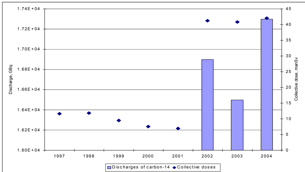
Figure 3 Reported atmospheric discharges of ^{14}\text{C} from Cap de la Hague and implied total collective dose to the EU population truncated at 500 y from exposure to all reported atmospheric discharges
