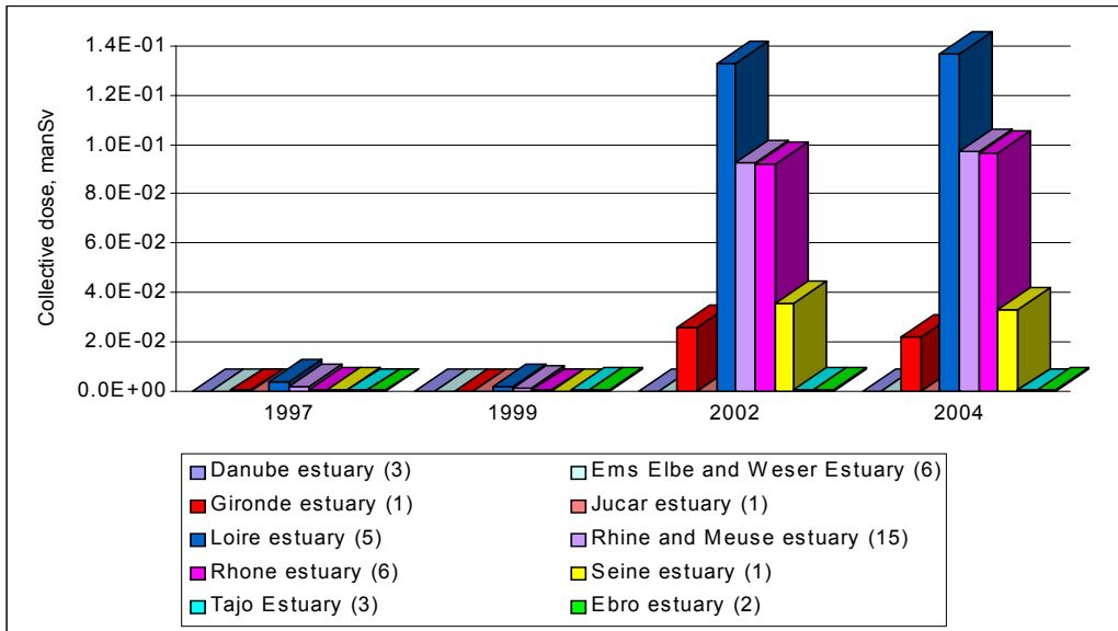
Figure 10 Implied collective doses truncated at 500 y to the EU population arising from reported marine discharges from inland sites (for some sites reported discharges did not include 14 C prior to 2002). Legend includes number of sites in brackets
