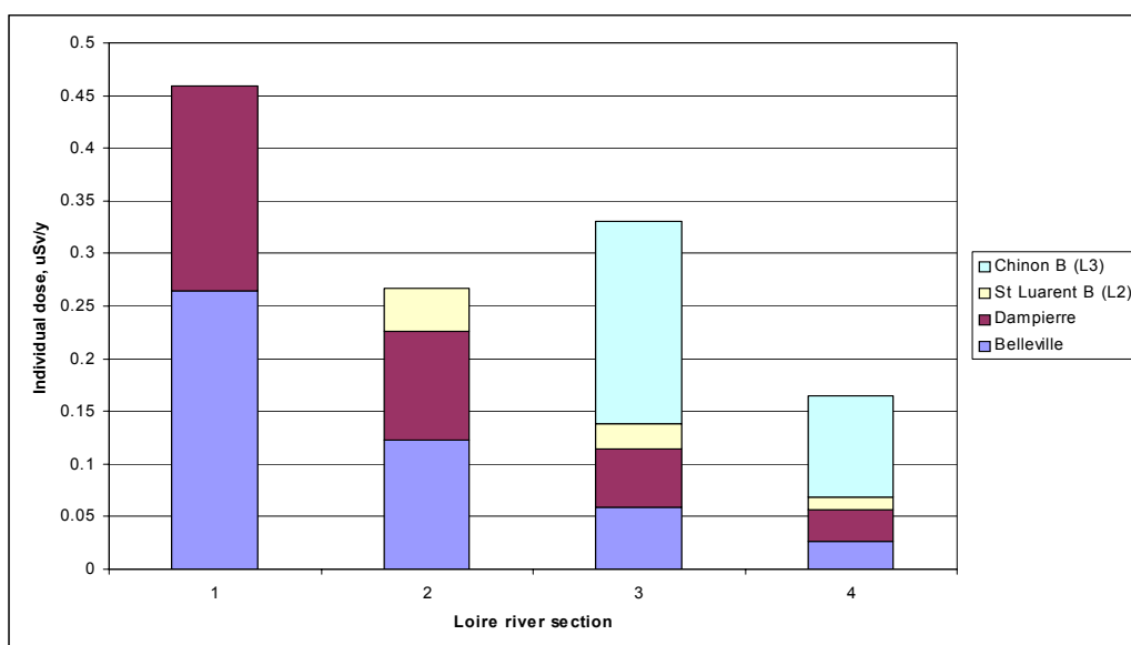
Figure B1 Representative adult critical group doses for different sections of the River Loire showing the contribution of reported discharges from key sites for 1996
