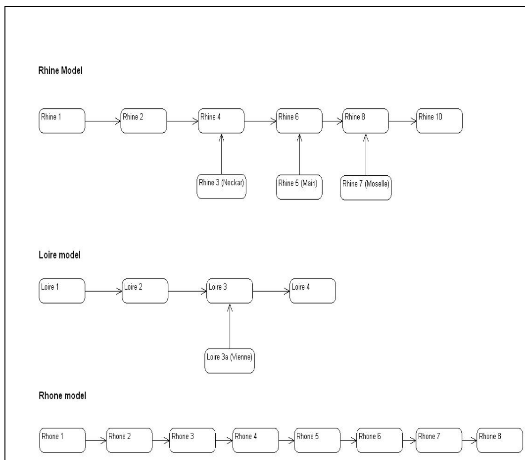
Figure 1 Layout of rivers modelled (section 9 of the Rhine river system, i.e., the river Lippe, was not considered as no discharges into this section of the river were reported)
