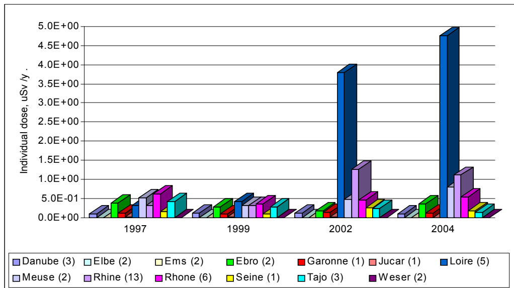
Figure 16 Representative adult critical group doses arising from reported discharges into each river system (for some sites reported discharges did not include ^{14}\text{C} prior to 2002). Legend includes number of sites in brackets
