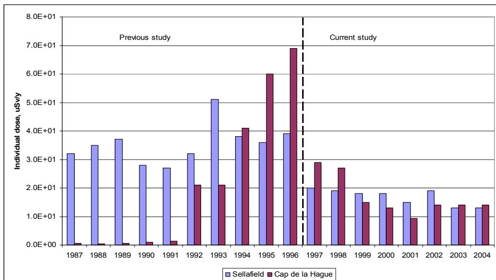
Figure 5 Representative adult critical group doses at the Sellafield and Cap de la Hague sites, based on reported atmospheric discharges, for a member of the critical group living 500 m away from the point of release. For Cap de la Hague reported discharges did not include ^{14}\text{C} in the years 1987, 1991, 1997 and 1999
