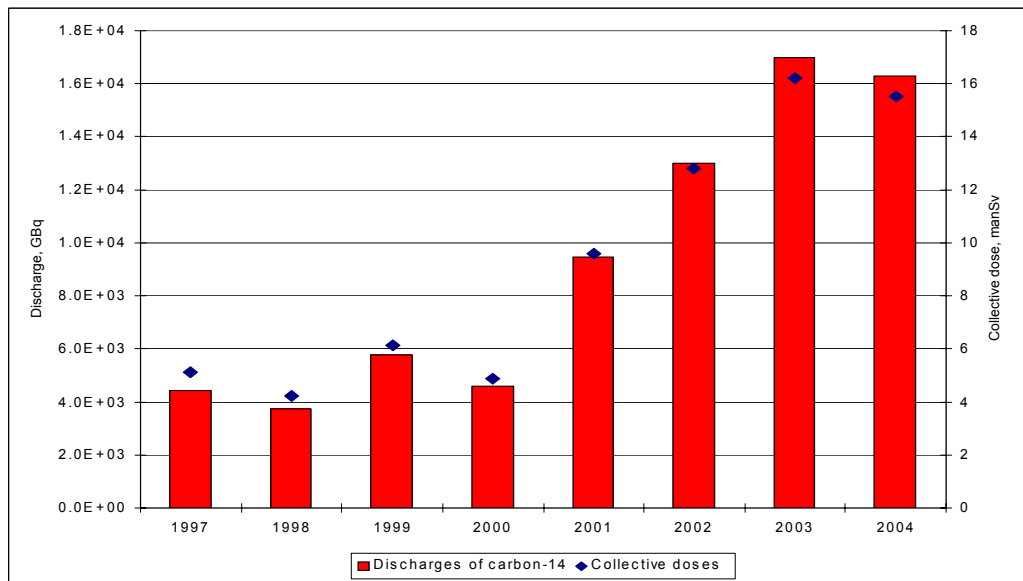
Figure 13 Reported liquid discharges of ^{14}\text{C} from Sellafield and implied total collective dose to the EU population truncated at 500 y from exposure to all reported liquid discharges
