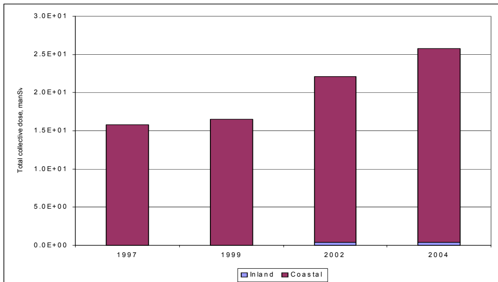
Figure 7 Implied collective doses truncated at 500 y to the EU population arising from reported marine discharges from all sites (for some sites reported discharges did not include ^{14}\text{C} prior to 2002)
