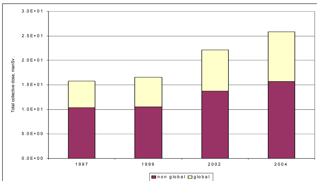
Figure 11 Implied collective doses truncated at 500 y to the EU population arising from reported marine discharges from all sites, showing contributions from 'global' and 'non-global' ('first pass') components (for some sites reported discharges did not include ^{14}\text{C} prior to 2002)
