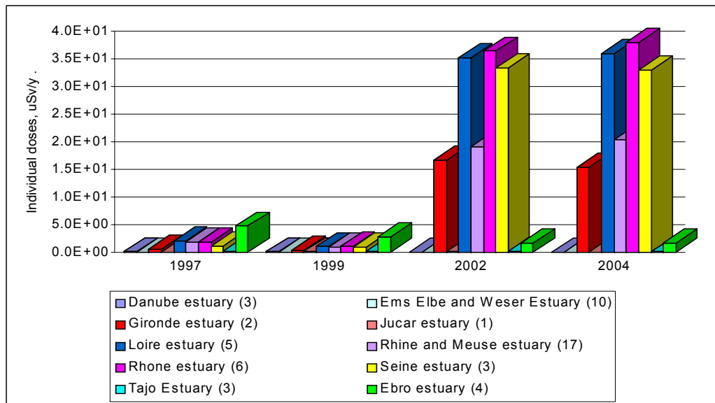
Figure 17 Representative adult critical group doses arising from reported discharges to each river estuary (for some sites reported discharges did not include ^{14}\text{C} prior to 2002). Legend includes number of sites in brackets
