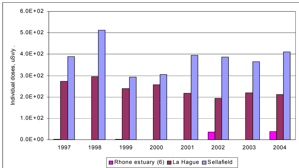
Figure 18 Representative adult critical group doses arising from reported marine discharges for selected sites (for sites on the Rhone reported discharges did not include ^{14}\text{C} prior to 2002)
