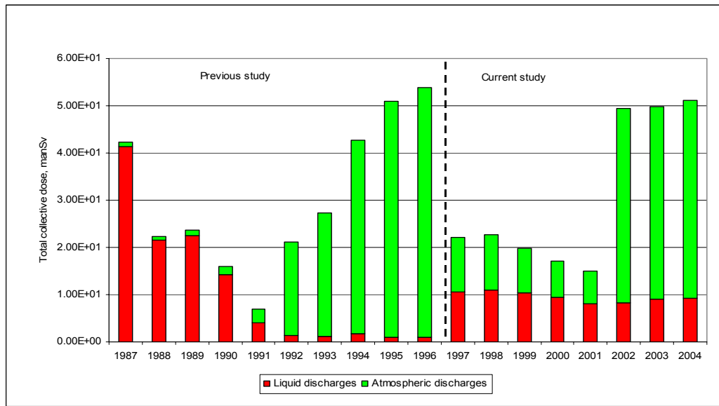
Figure 20 Implied total collective dose truncated at 500 y to the EU population arising from reported discharges from the Cap de la Hague site (reported discharges did not include 14 C from 1987 to 1991 and 1997 to 2001 for atmospheric releases and from 1987 to 1996 for liquid releases)
