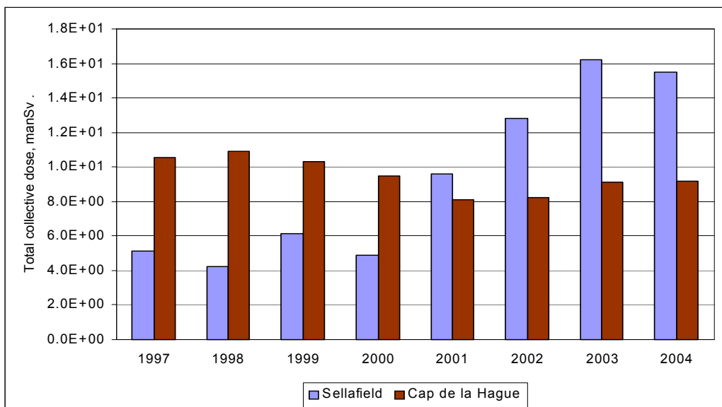
Figure 8 Implied collective doses truncated at 500 y to the EU population arising from reported marine discharges from Sellafield and Cap de la Hague (reported discharges included ^{14}\text{C} )
