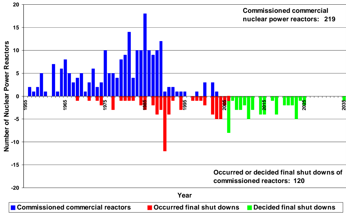
Figure 2.2: Timeline of power reactor commissioning and closure
