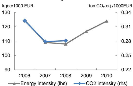
Graph II.1.10: Bulgaria - Energy and carbon intensity of households
