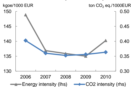
Graph II.10.7. Luxembourg - Energy and carbon intensity of the economy
