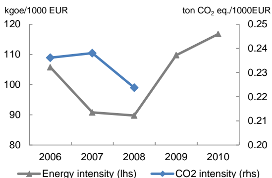
Graph II.9.10: Lithuania - Energy and carbon intensity of households
