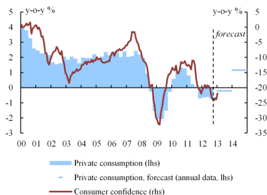
Graph I.11: Private consumption and consumer confidence, EU
