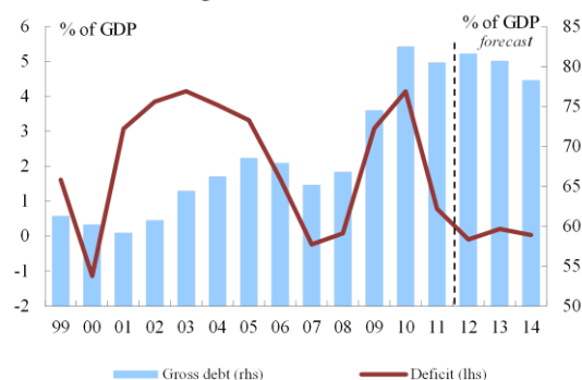
Graph II.5.2: Germany - General government gross debt and deficit
