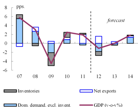
Graph II.3.1: Czech Republic GDP growth and contributions
