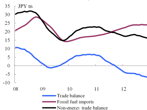
Graph II.31.1: Japan - Trade balance, fossil fuel imports and non-energy trade balance (cumul. over 12-months)
