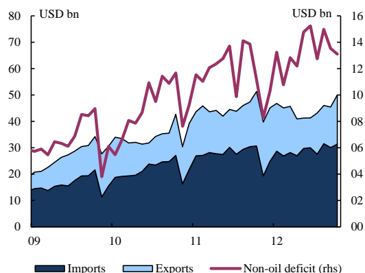
Graph II.33.2: Russia - trade
