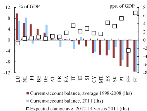
Graph I.12: Current-account balances, euro-area and Member States
