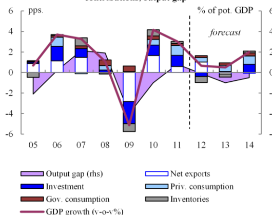
Graph II.5.1: Germany - GDP growth and contributions, output gap
