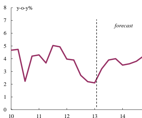
Graph II.33.1: Russia - GDP growth
