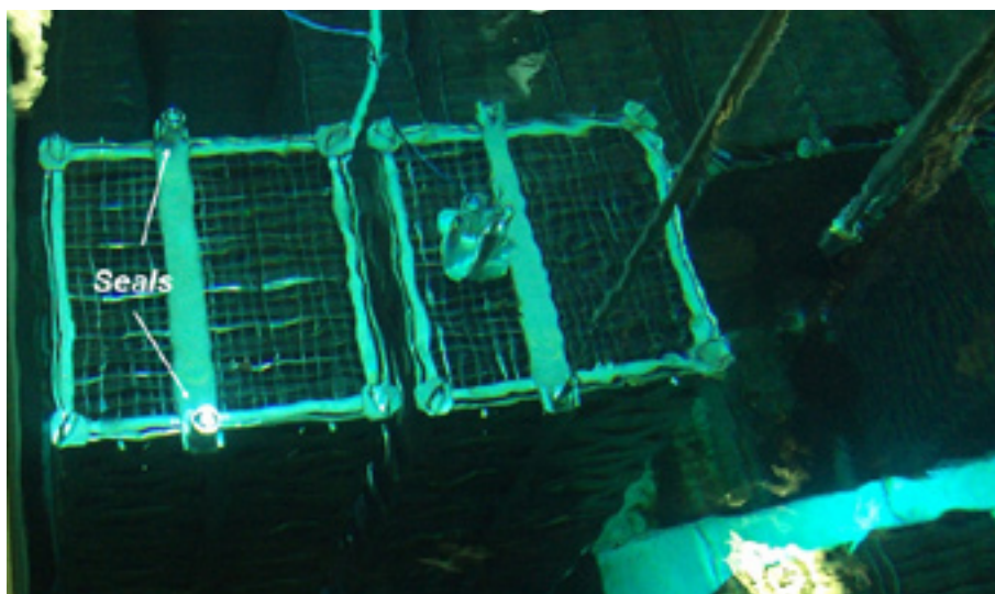
JRC Kanupp sealing system for nuclear fuel: left rack already sealed, right rack is being sealed
