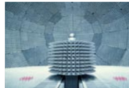
Target calibration in the EMSL microwave laboratory.
