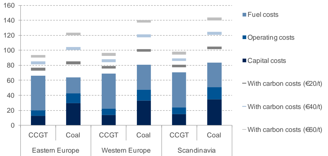
Figure 6: LCOE for an installation in 2020, per region and cost component (€/MWh)
