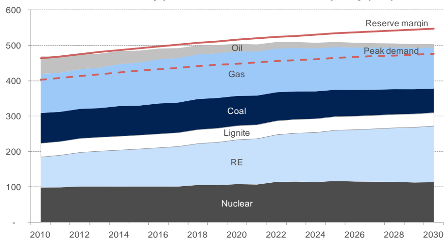
Figure 3: EU-27 + Iceland + Norway peak demand and available capacity (GW)
