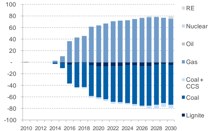
Figure 15: Difference in power generation (TWh)
