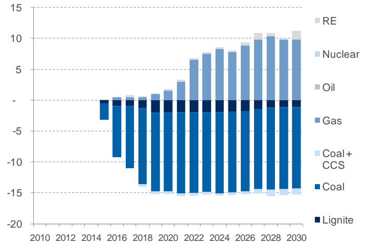
Figure 13: Difference in installed capacity (GW)
